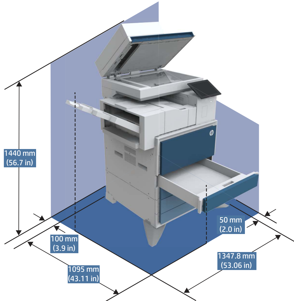
Figure 1-11 Printer, dual cassette feeder, and inner finisher dimensions (fully open)
