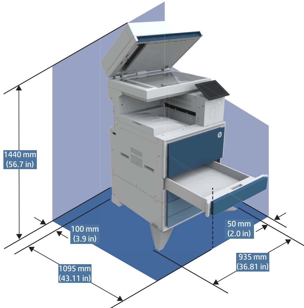
Figure 1-10 Printer and dual cassette feeder dimensions (fully open)
