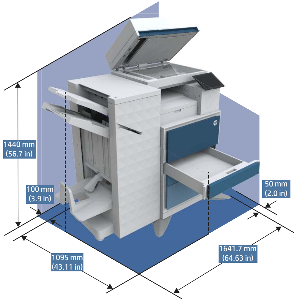
Figure 1-12 Printer, booklet finisher, and 2K high-capacity input dimensions (fully open)
