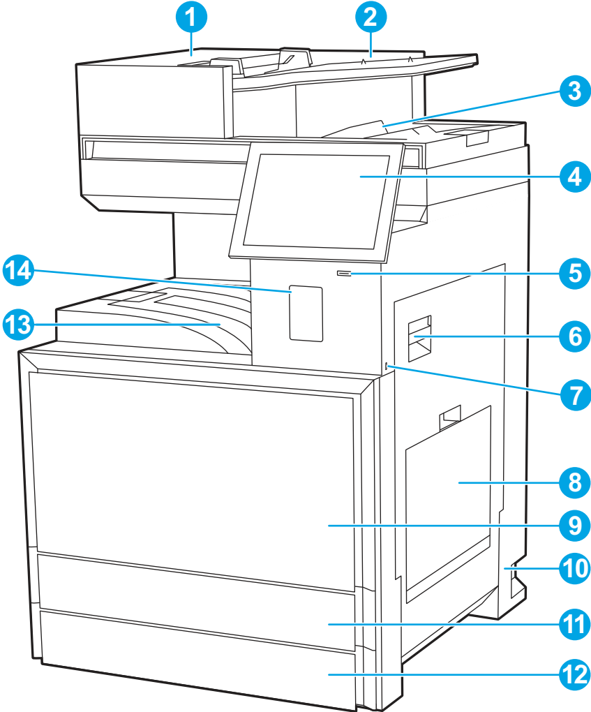
Figure 1-6 Printer front view
