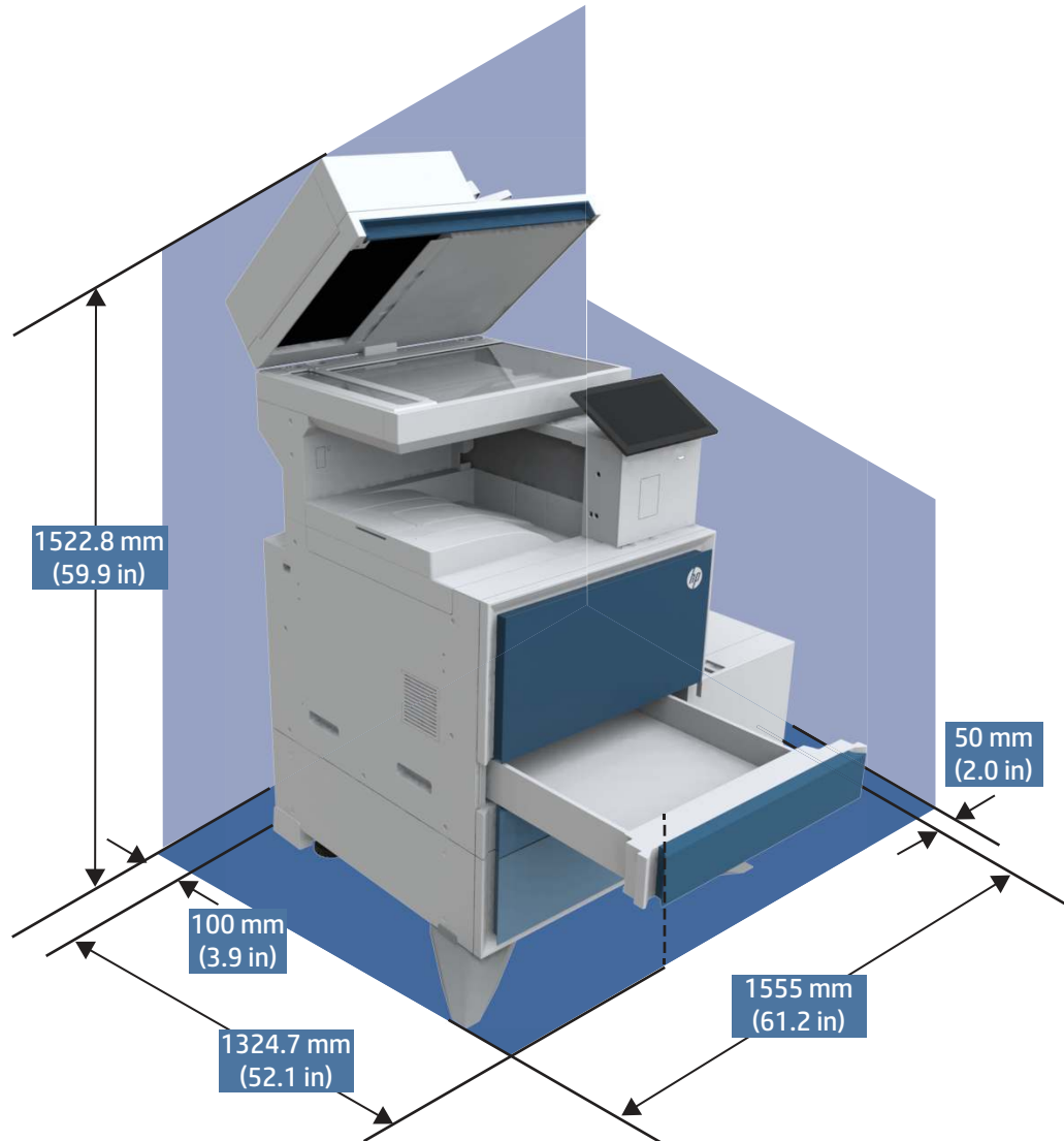
Figure 1-14 Printer, 2K high-capacity input, and side high-capacity input dimensions (fully open)
