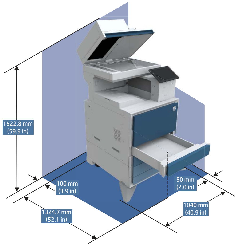
Figure 1-10 Printer and dual cassette feeder dimensions (fully open)
