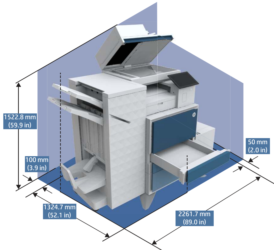
Figure 1-13 Printer, booklet finisher, 2K high-capacity input, and side high-capacity input dimensions (fully open)
